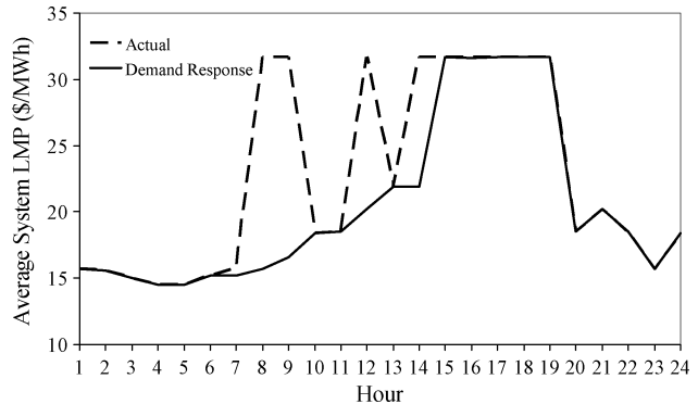
Fig. 5. Average system LMP.
